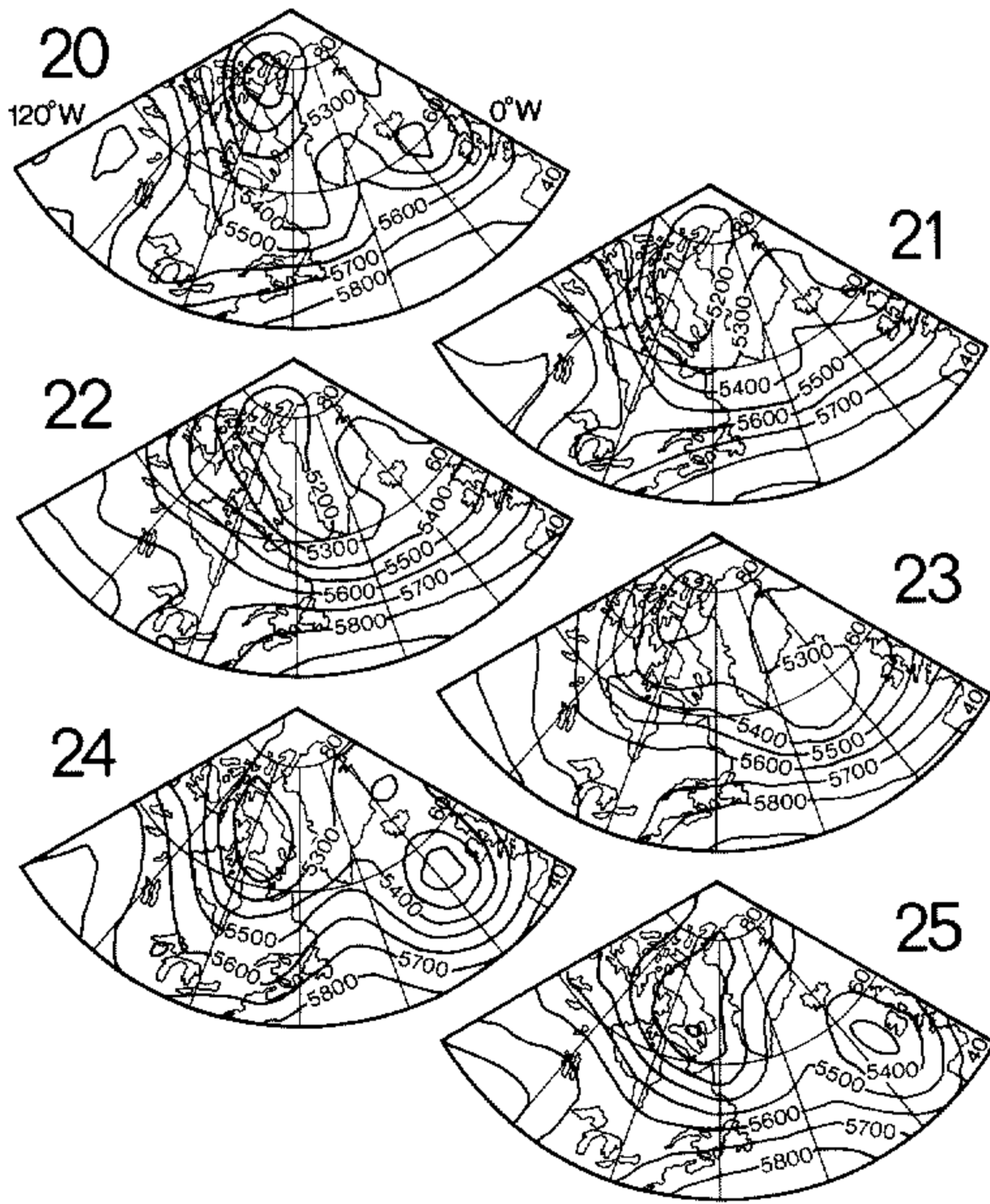
Figure 6. The 500 mb geopotential heights corresponding to the IPV maps shown in Fig. 5. They are for the period 20–25 September 1982 and the region 40°N–90°N and 120°W–0°W. The contour interval is 100 m.
